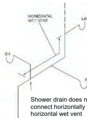
Noncompliant Horizontal Wet Vent
