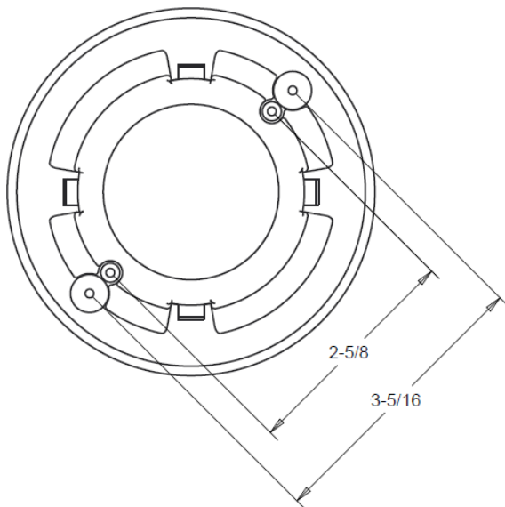
Item # 63694, Long Barrel (no grate)
