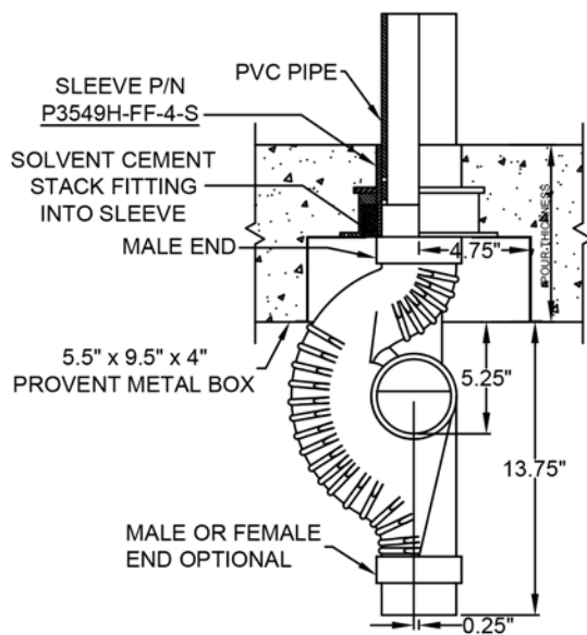
P3549H-FF-4-S 3" Stack Top is Male
