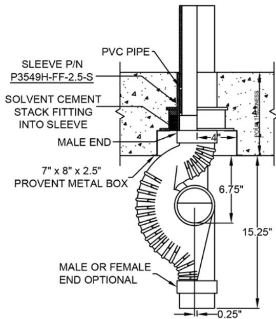
P3549H-FF-2.5-S 3" Stack Top is Male
