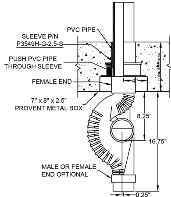
P3549H-G-2.5-S 3" Stack Top is Female
