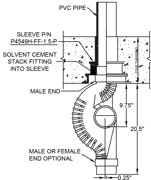
P4549H-FF-1.5-P 4" Stack Top is Male
