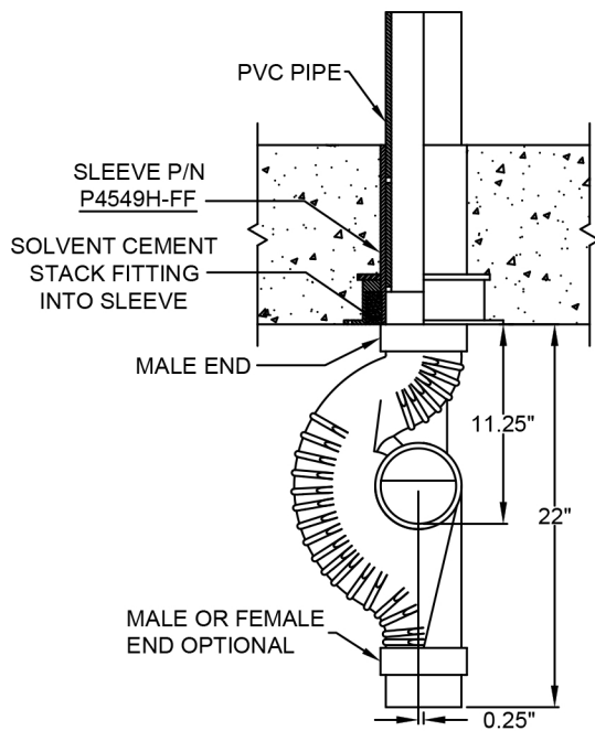
P4549H-FF 4" Stack Top is Male
