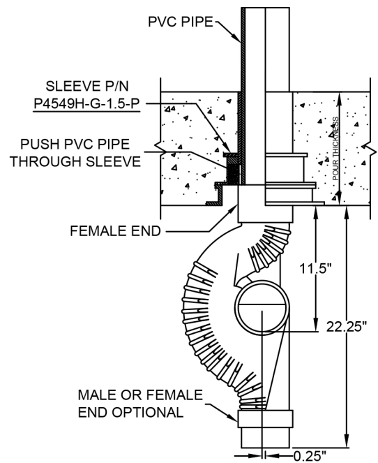
P4549H-G-1.5-P 4" Stack Top is Female
