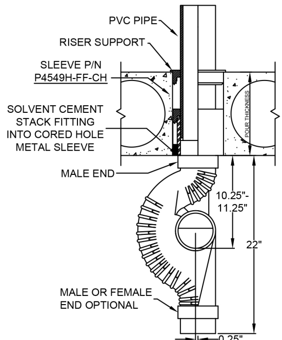
P4549H-FF-CH 4" Stack Top is Male
